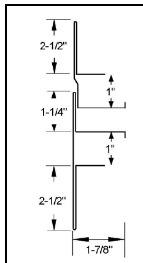
DFXS-1375 EXPANSION JOINT
