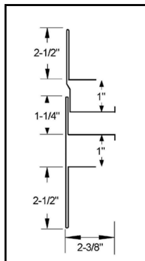
DFXS-15375 EXPANSION JOINT
