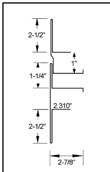
DFXS-2375 EXPANSION JOINT BRAND X METALS, INC.
