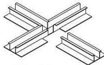
4-Way Intersection (Mitered or Notched)
