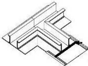
Tee Intersection (Mitered or Notched)
